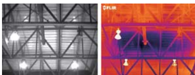
Roofing - Infrared testing is used to detect water damage & leaks beneath the surface of the roof allowing the opportunity repair the section before it continues to spread.
