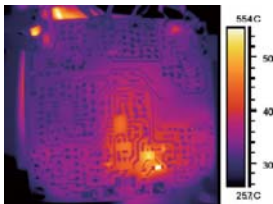
Wafer Board - This is an annealing process for wafers. Thermography can quickly identify thermal irregularities on critical parts.
