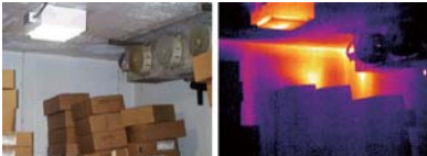
Freezer – Poor insulation in a walk-in cooler
